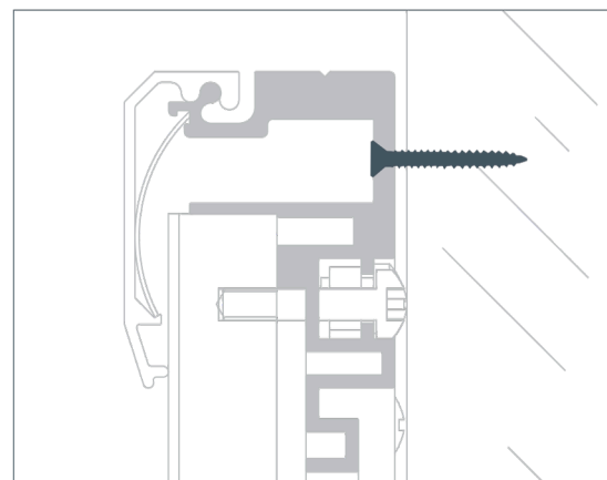
Wall mount diagram
